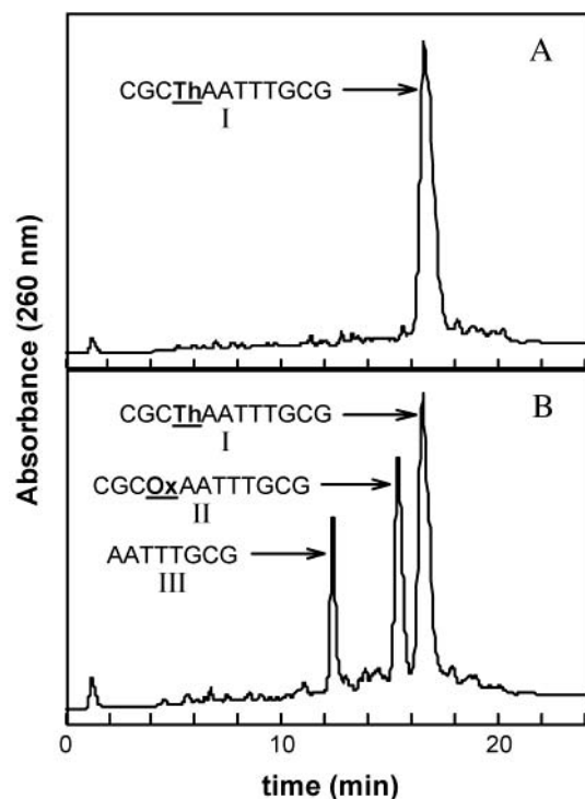
Figure 2. (A) Chromatogram of the Dickerson dodecamer containing thiazole C-nucleoside (Th); MALDI ( M - H ) - 3593, (calcd) 3593. (B) Chromatogram of the Dickerson dodecamer containing thiazole N -oxide C-nucleoside (Ox); I. MALDI ( M - H ) - 3593, (calcd) 3593; II. MALDI ( M - H ) - 3613 (calcd) 3609; III. MALDI ( M - H ) - 2426 (calcd) 2422. Conditions: Hydrocell NS 1000 (anion exchange) 150 × 4.6 mm column; solvent A 25 mM CHES pH 8, 30% MeOH; solvent B 25 mM CHES/1 M (NH 4 ) 2 SO 4 pH 8, 30% MeOH; 0–100% B over 60 min, flow rate = 1 mL/min.
