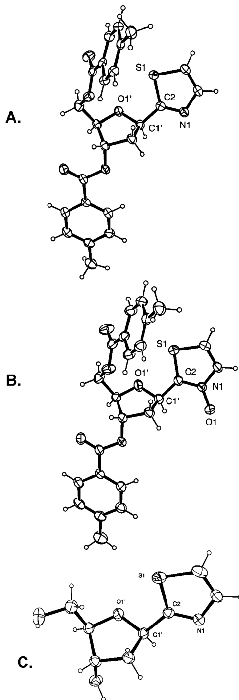
Figure 1. X-ray crystallography ORTEP diagrams of (A) 2-(3',5'- O - p -toluoyl-2'-deoxy- \beta -D-ribofuranosyl)thiazole, (B) 2-(3',5'- O - p -toluoyl-2'-deoxy- \beta -D-ribofuranosyl)thiazole- N -oxide, and (C) 2-(2'-deoxy- \beta -D-ribofuranosyl)thiazole.
